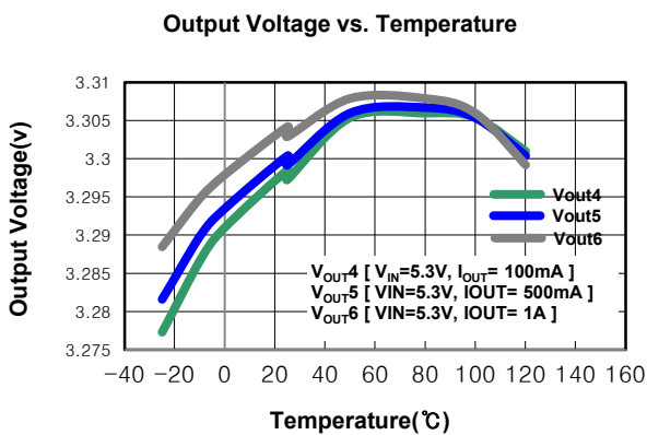
Graph 5 Electrical Characteristics Curves
